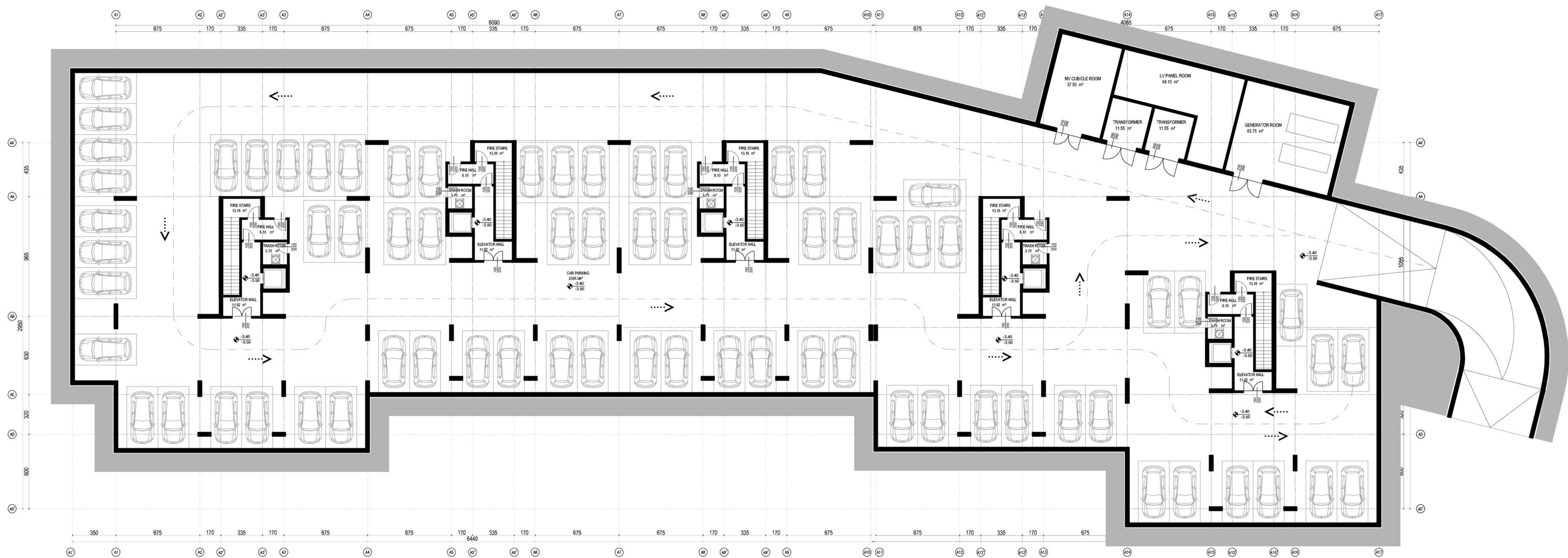
BLOCK A 1st BASEMENT FLOOR PLAN 1/200
