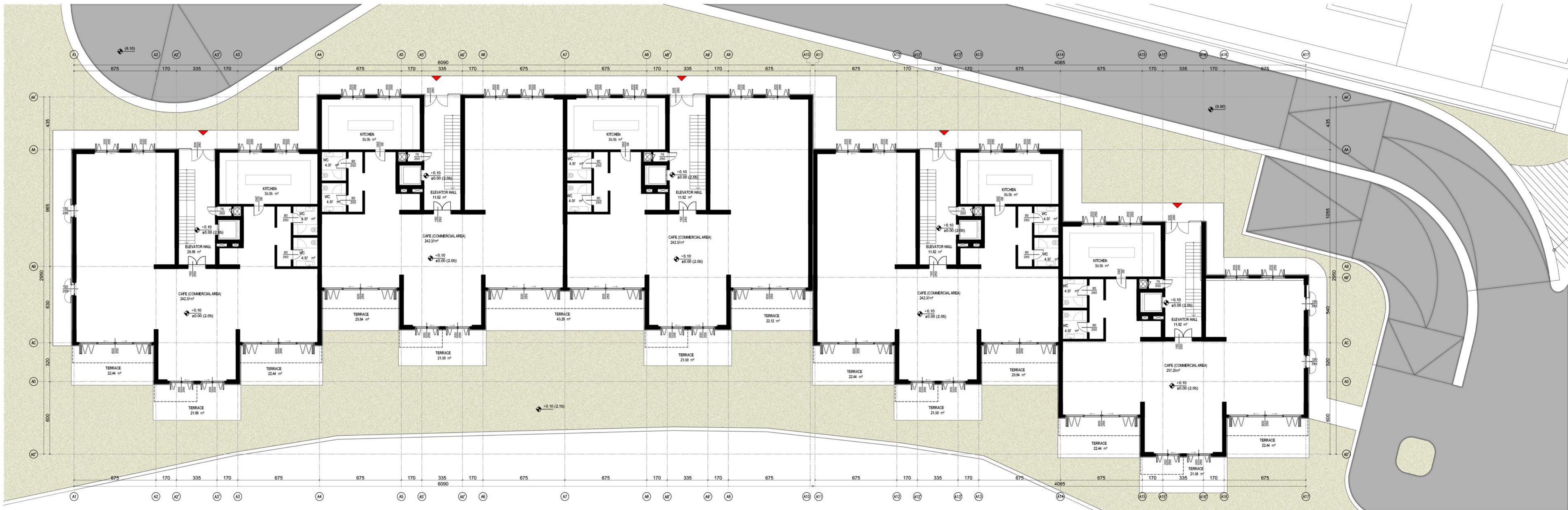
BLOCK A GROUND FLOOR PLAN 1/200
