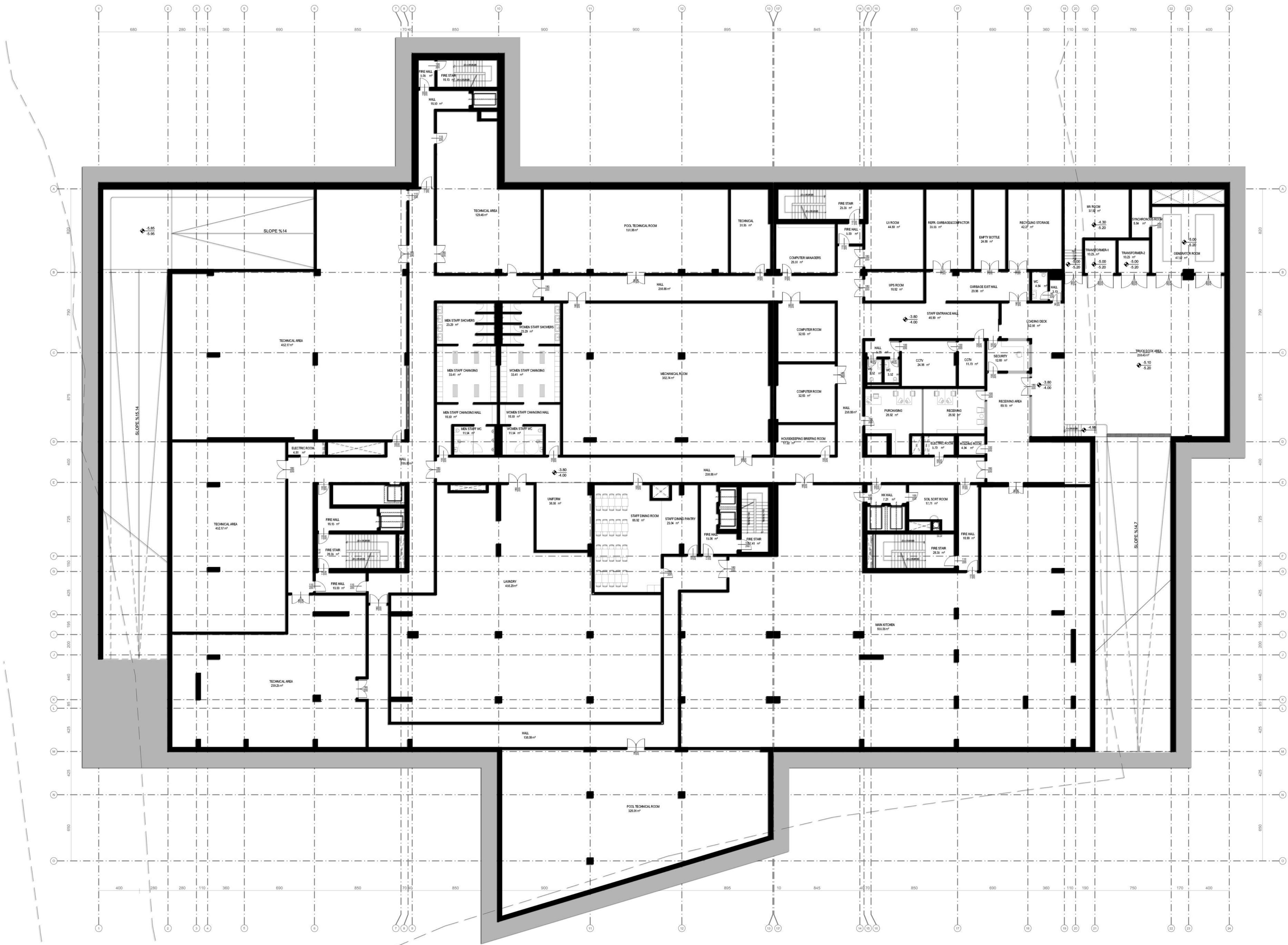
HOTEL BLOCK 1st BASEMENT FLOOR PLAN 1/200
