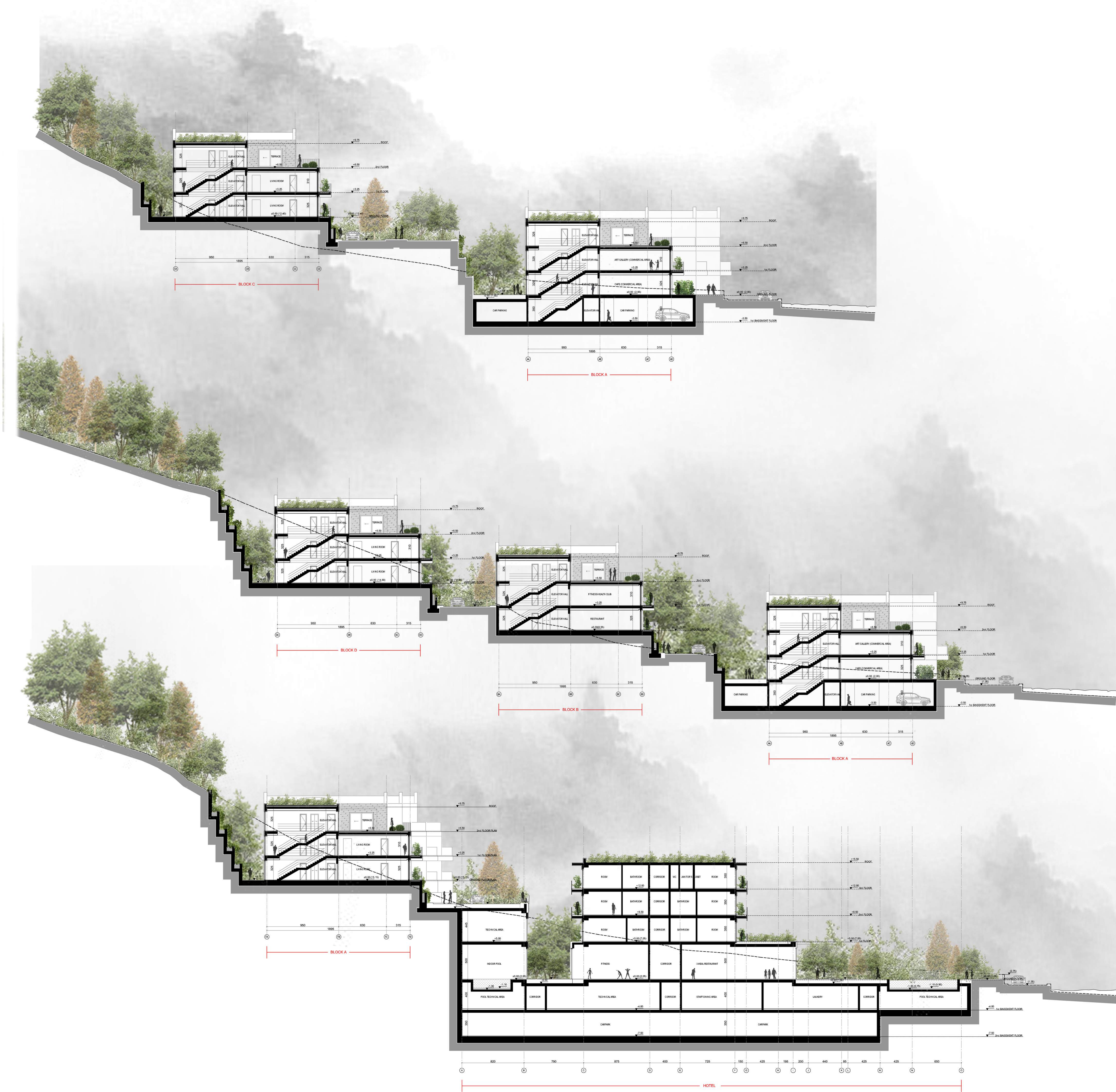
SECTION 1-1
